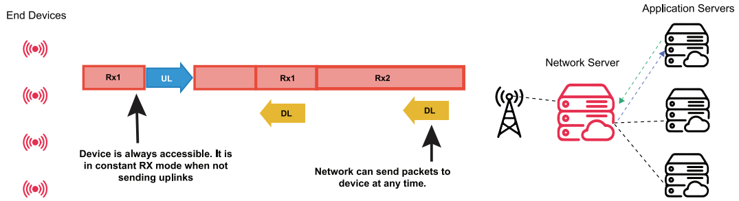
Figure 2.29: LoRaWan Class C operation
