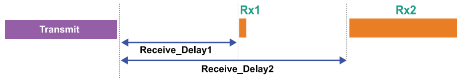
Figure 2.26: LoRaWAN Class A operation when a data packet is received in the second receive window
