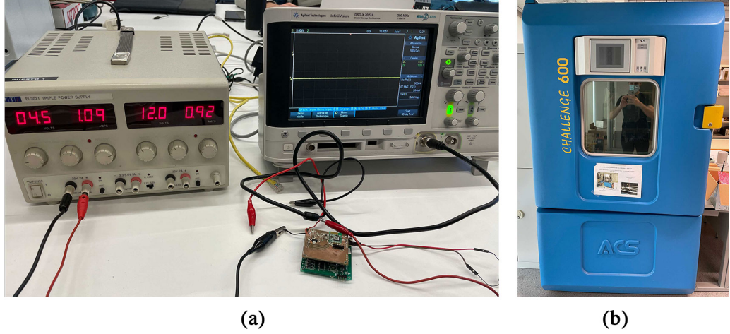
Figure 3.9: Test bench: (a) The circuit is powered and connected to a PC for monitoring and data analysis using Bluetooth. (b) the climate chamber used for characterization
