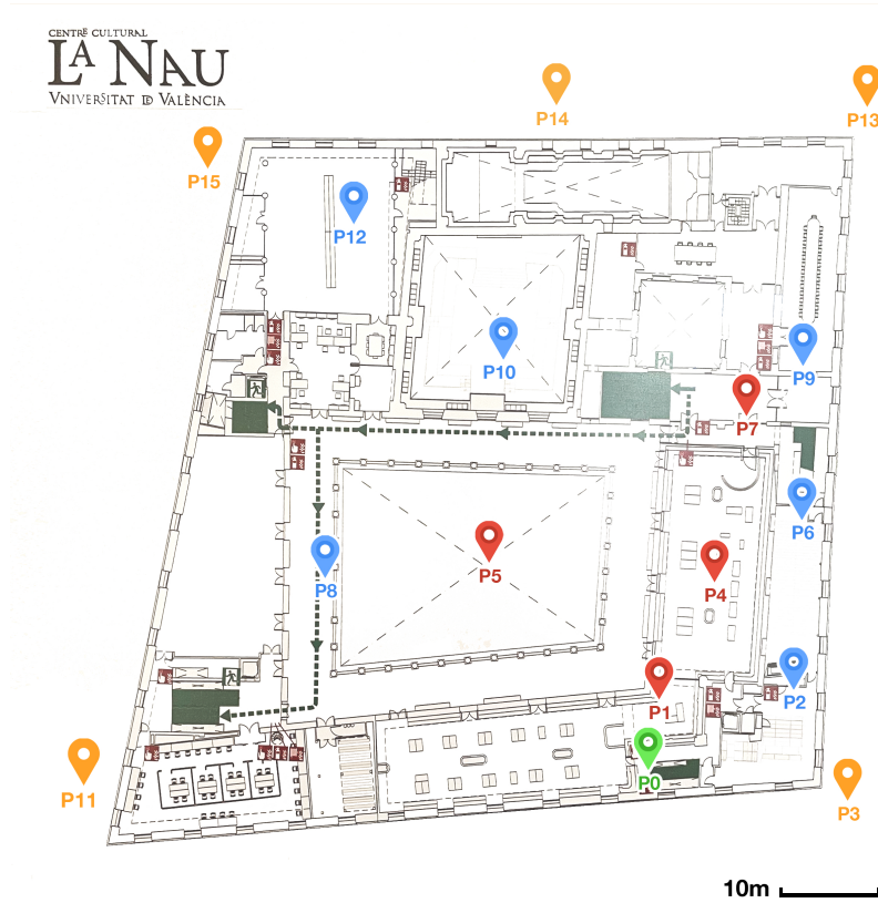
Figure 5.10: Plan of the cultural Centre La Nau showing the position of the gateway (P0) and the location of different measurement points (P1 to P15) where the LoRa MC end-nodes were located. Red, blue and orange colors refer to the ground floor, first floor and grand floor, but outdoors, respectively.
