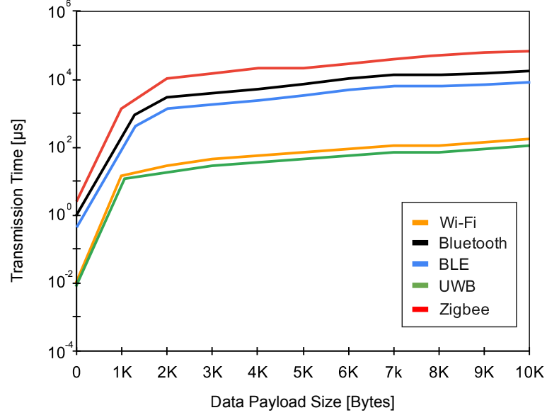
Figure 2.6: Comparison between transmission time and data size in short-range communication protocols
