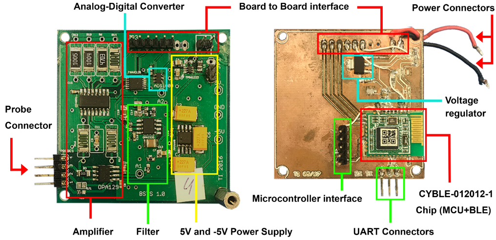
Figure 3.3: BLE moisture device circuit: analog and digital boards. The size of the circuit when the boards are connected: 5.7 cm × 5.3 cm × 1.5 cm [184]
