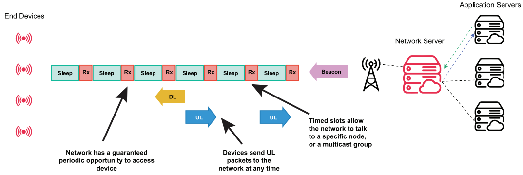
Figure 2.27: LoRaWAN Class B beaoning operations
