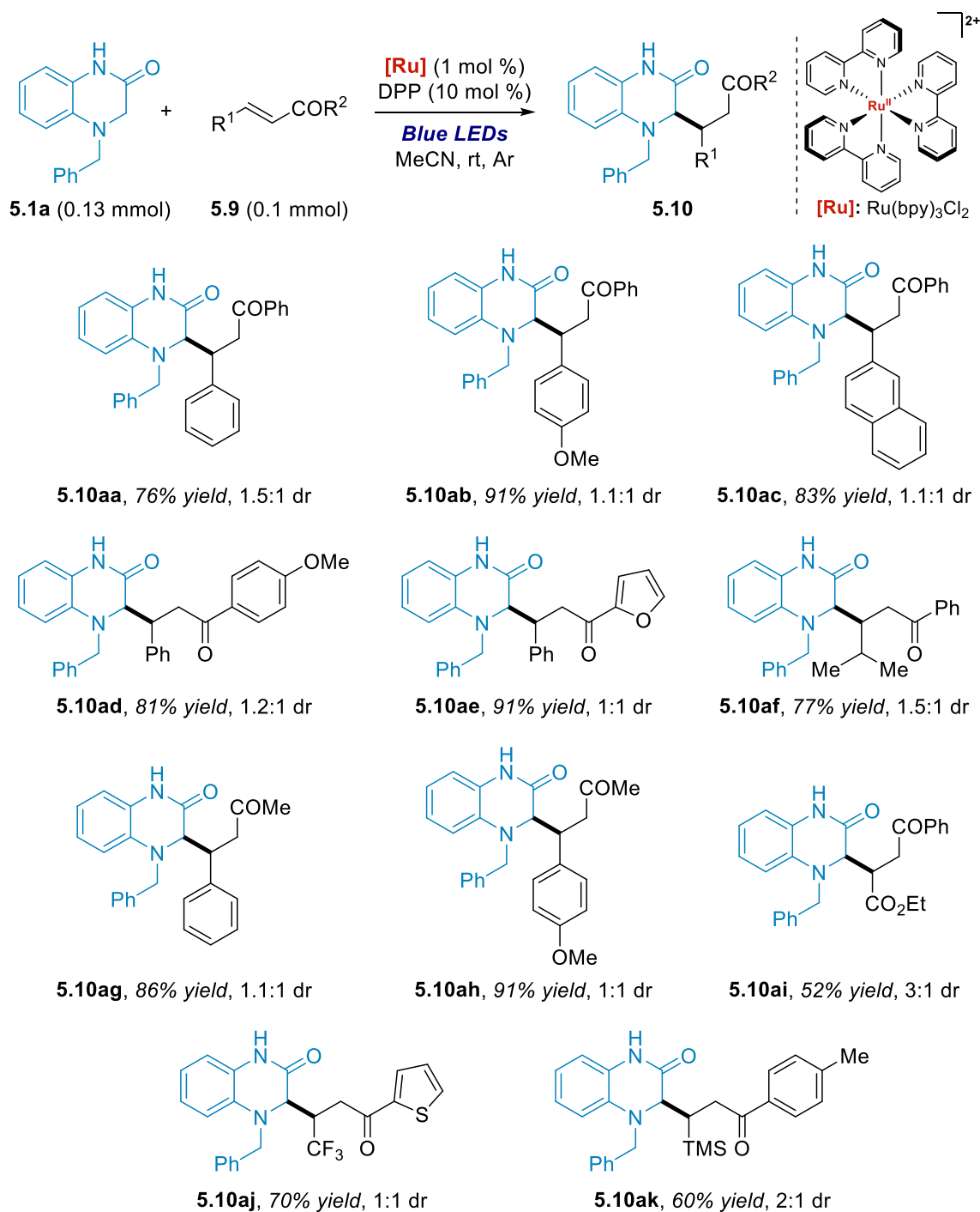
Scheme 5.17: Scope of the reaction using 4-benzyl-3,4-dihydroquinolin-2-one ( 5.1a ) and different \alpha,\beta -unsaturated ketones ( 5.9 ). a
