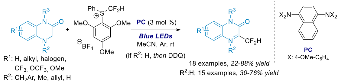
Figure 36: Difluoromethylation of 3,4-dihydroquinoxalin-2-ones through visible-light photoredox catalysis (Liu).
