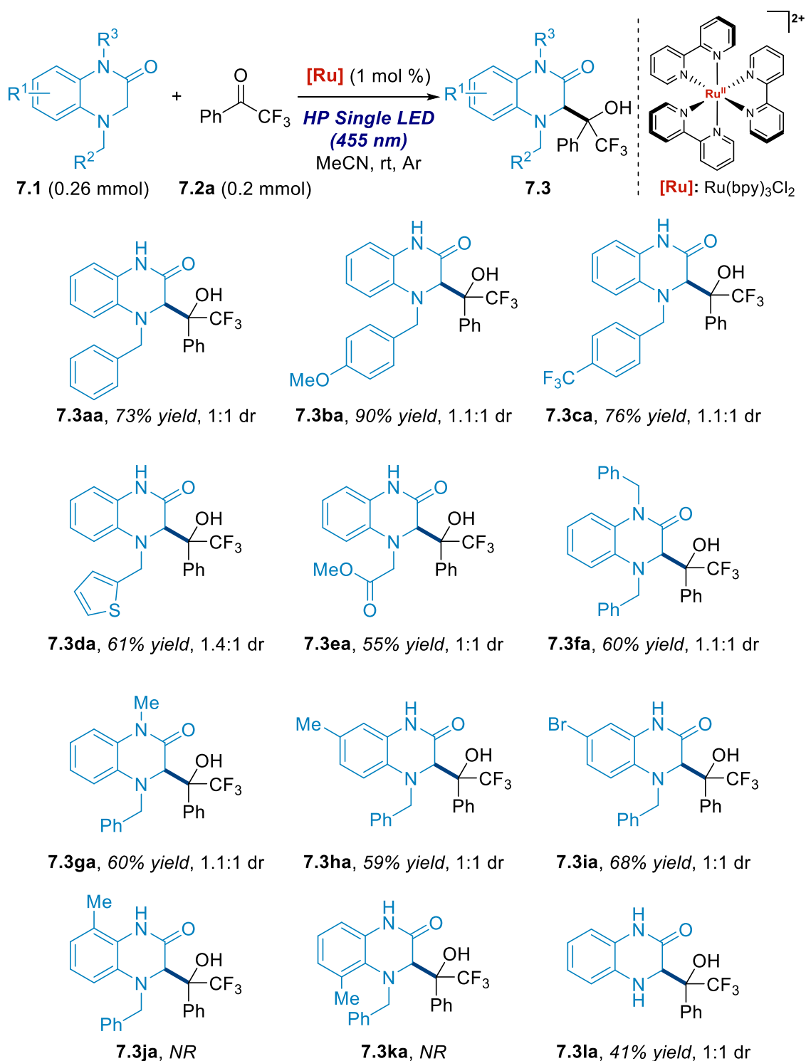
Scheme 7.10: Scope of the reaction using different 3,4-dihydroquinoxalin-2-ones ( 7.1 ) and trifluoroacetophenone ( 7.2a ). a
