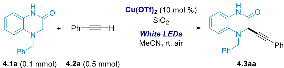
Scheme 4.9: Final adjustments in the reaction between 4.1a and 4.2a using Cu(OTf) 2 , SiO 2 and MeCN.
