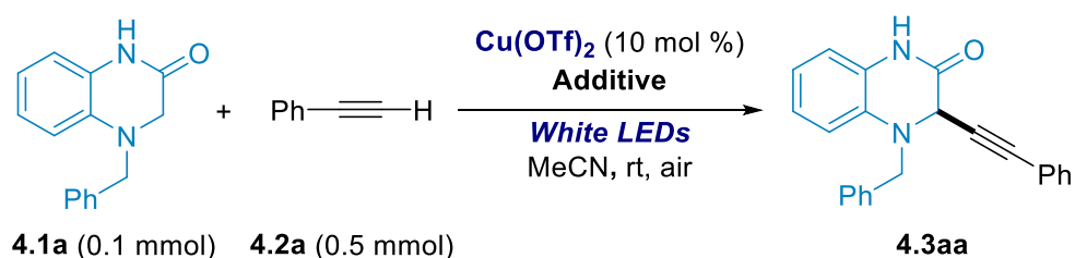
Scheme 4.8: Evaluation of additives in the reaction between 4.1a and 4.2a using Cu(OTf) 2 and MeCN.
