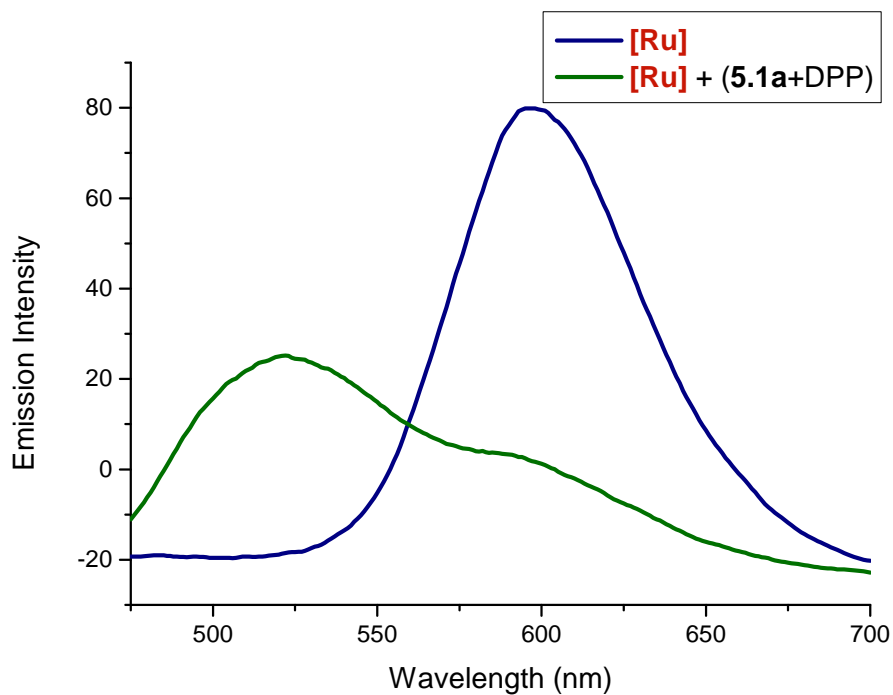
Figure 5.3: Emission spectra of a solution containing 0.02 mM of \text{Ru}(\text{bpy})_3\text{Cl}_2 (A) and a premixed blend of 5.1a and DPP.
