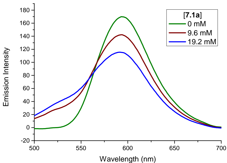
Figure 7.6: Emission spectra of different solutions containing 0.02 mM of Ru(bpy) 3 Cl 2 (A), 9.6 mM of 7.2a and varying amounts of 7.1a.
