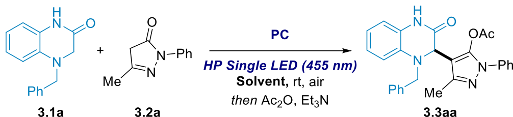
Scheme 3.5: Overview of the model reaction to carry out the optimization of the reaction conditions.
