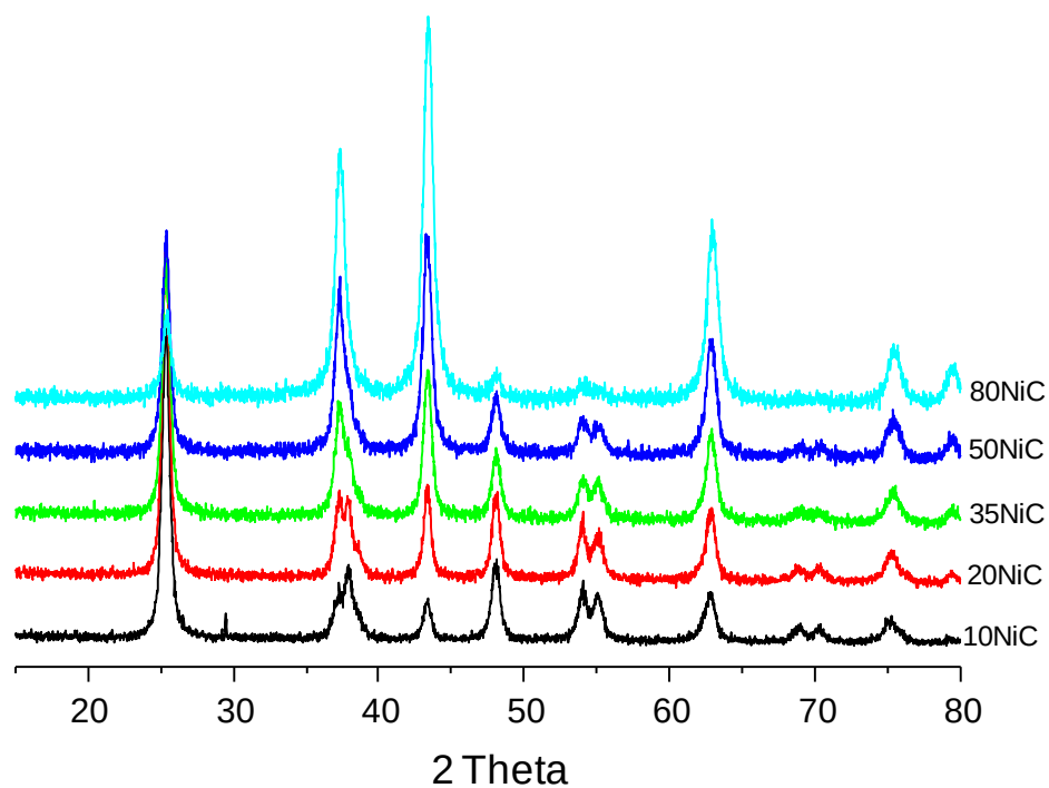
Figure S3. XRD patterns of NiO/TiO 2 catalysts (C-series).
