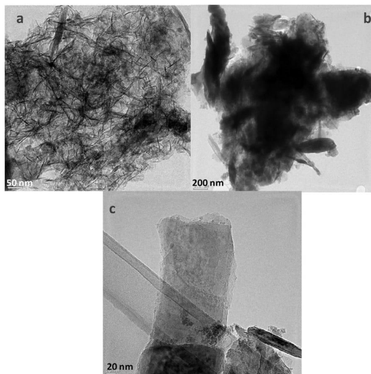
Fig. 2. TEM images of sample SL-550, the ferric sludge calcined at 550 °C, showing different morphologies.
