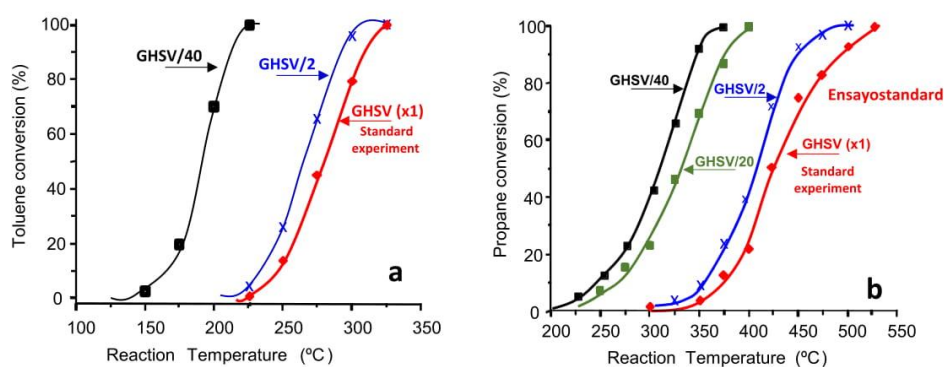
Fig. 4. Variation of the toluene conversion (a) and propane conversion (b) with the reaction temperature for the ferric sludge calcined at 550 °C, SL-550. Influence of the space velocity on the catalytic activity. Reaction conditions in text.
