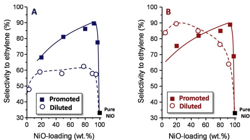
Fig. 1. Selectivity to ethylene in the ODH of ethane as a function of NiO-loading for promoted/diluted NiO catalysts: A) xNb-Ni-O and xNiO/Nb 2 O 5 -series; B) xTi-Ni-O and xNiO/TiO 2 -series. Reaction conditions in text.
