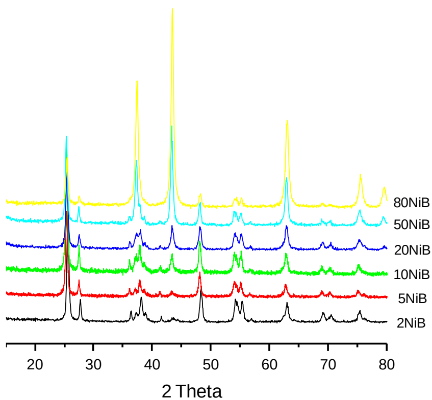
Figure S2. XRD patterns of NiO/TiO 2 catalysts (B-series).
