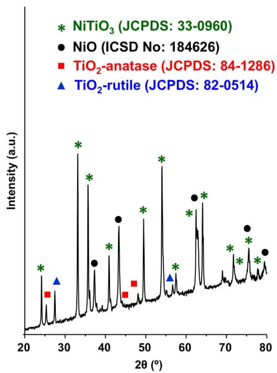
Figure S5. XRD pattern of 50Ni-Ti-O sample calcined at 700 °C for 4 h.
