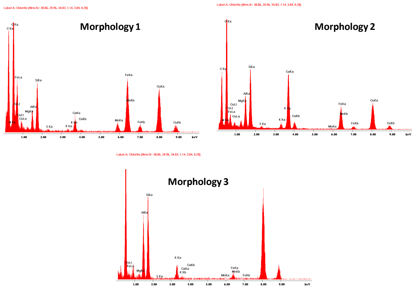
Figure S1. EDX of the different morphologies observed in the sludge calcined at 550°C (SL-550).
