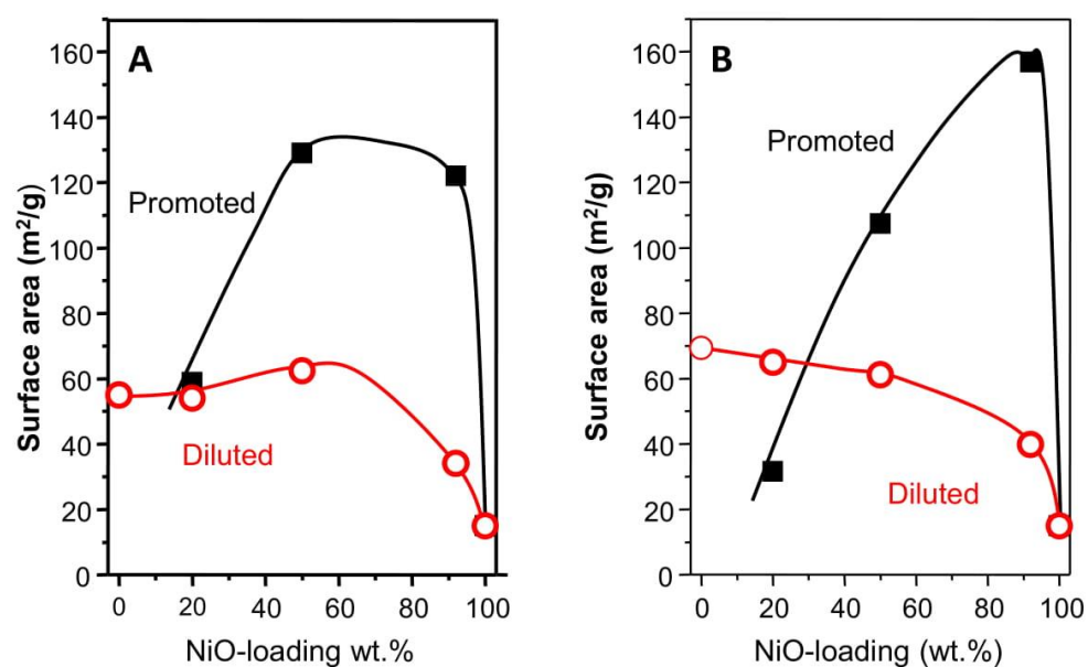
Figure S2. Variation of BET surface area with NiO-loading for promoted and diluted NiO catalysts.
