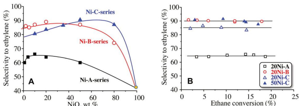
Fig. 1. Catalytic performance of NiO/TiO 2 catalysts: a) Variation of selectivity to ethylene (at ethane isoconversion of 10%) with the NiO-loading for catalysts of Ni-A-, Ni-B- and Ni-C-series; b) Variation of selectivity to ethylene with ethane conversion at different contact times, W/F, in the range of 1–12 g cat h -1 mol C 2 -1 .
