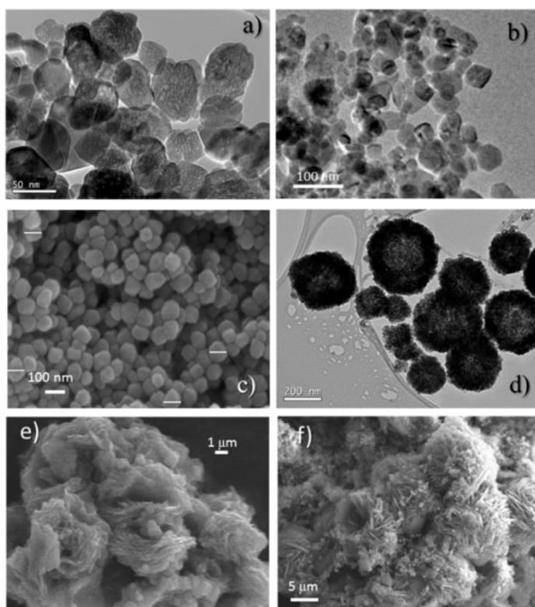
Figure 6. Representative EM images for the (a) Few200, (b) Few450, (c) Fe-HT, (d) Fe-ST1 and (e) Fe-ST2 fresh catalysts and (f) iron glycolate precursor of Fe-ST2.
