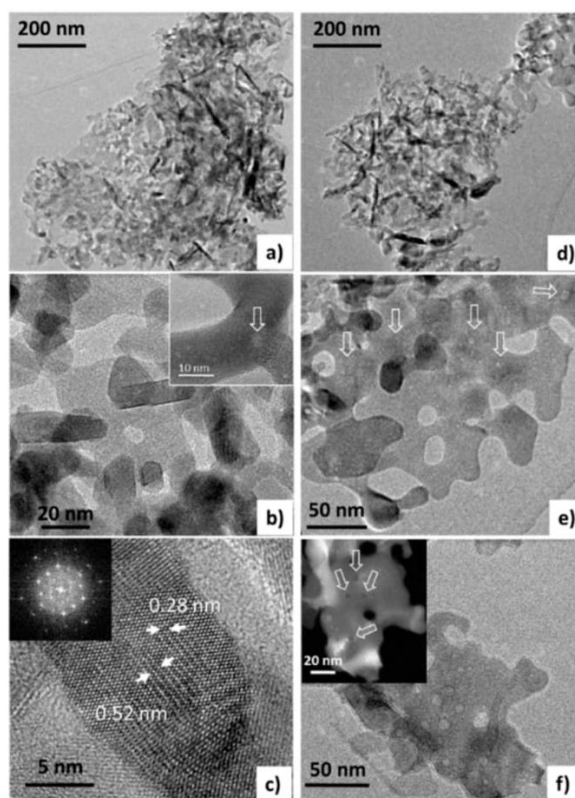
Figure 8. HRTEM images at different magnifications of the Fe-ST2 catalyst (a–c) before use and (d–f) after three catalytic cycles. Unfilled arrows indicate nanocavities. Insets: in (c) fast Fourier transform (FFT) coherent with indicated distances, which correspond to (111) and (220) interplanar distances of spinel structure; in (f) corresponding Scanning Transmission Electron Microscopy (STEM) image, in which nanocavities are clearly appreciated as black zones.
