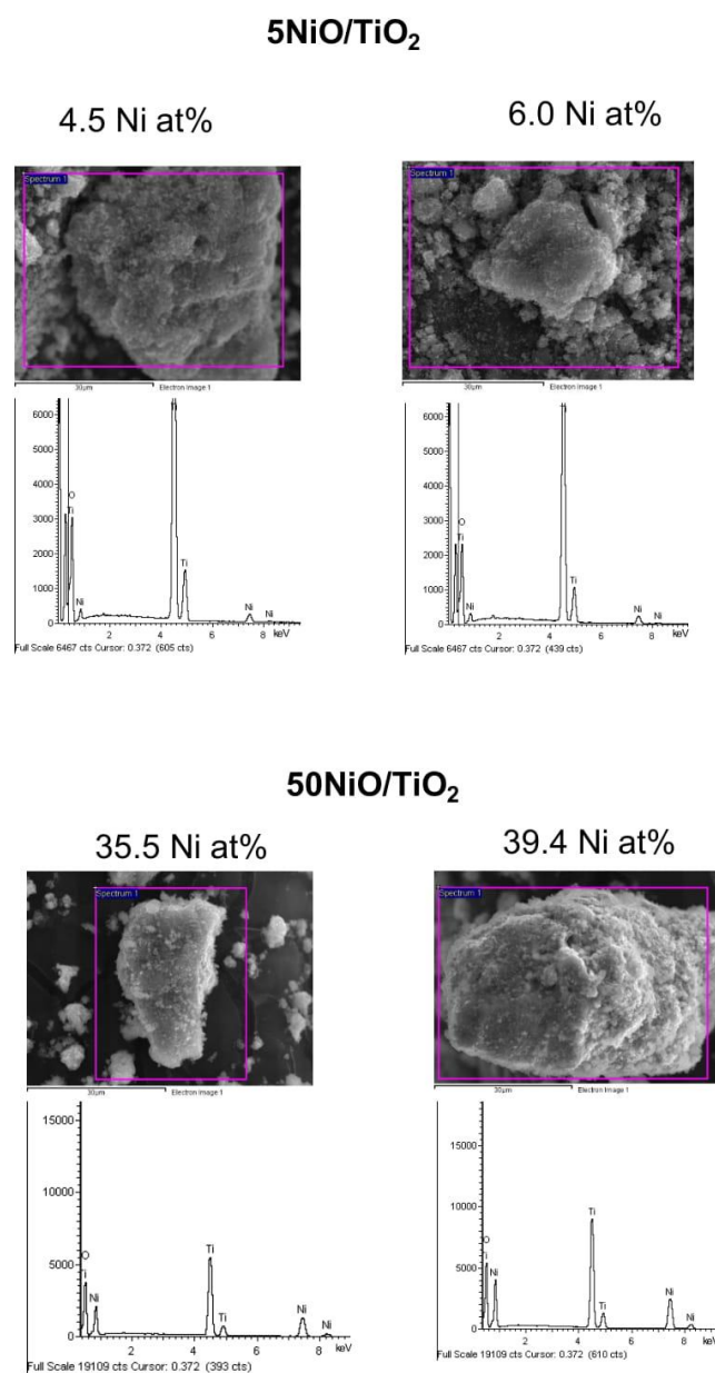
Figure S10. Scanning electron microscopy images and their corresponding EDX analyses of selected TiO 2 -supported NiO catalysts.
