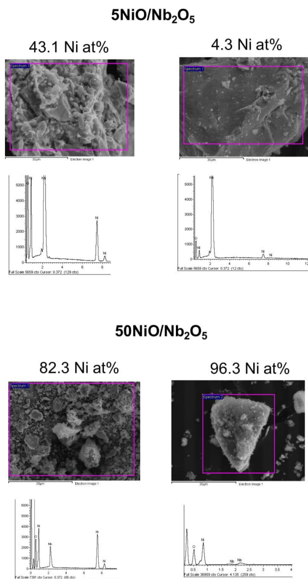
Figure S11. Scanning electron microscopy images and their corresponding EDX analyses of selected Nb 2 O 5 -supported NiO catalysts.
