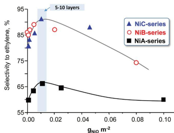
Fig. 7. Variation of the selectivity to ethylene with the theoretical NiO coverage (fixed conversion ≈ 10%). Note: Reaction temperature = 450 °C, C 2 H 6 /O 2 /He with a molar ratio of 3/1/26.
