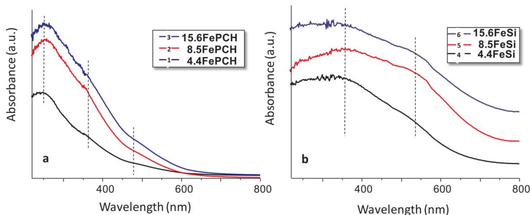
Fig. 2. Diffuse reflectance UV-vis spectra of xFe/PCH (a) and xFe/Si (b) catalysts.
