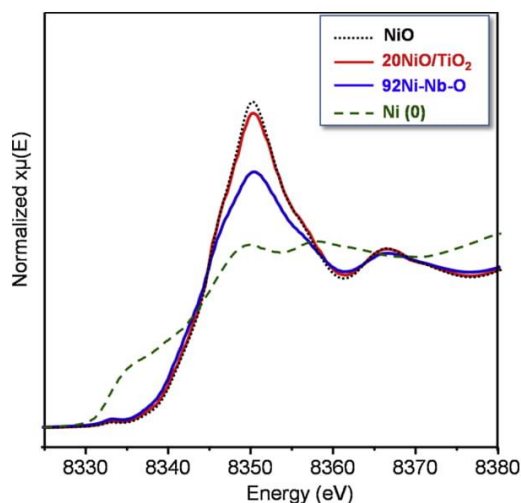
Fig. 6. XANES region of XAS spectra in the Ni K-edge of the most selective (sample 92Ni-Nb-O sample) and diluted (20NiO/TiO 2 sample) catalysts. For comparison, unmodified NiO and metallic nickel are also presented.
