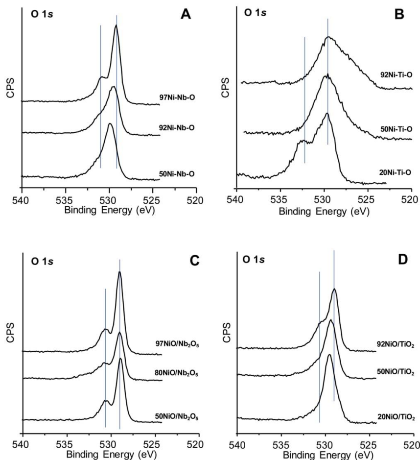
Fig. 5. O 1s core level spectra of promoted and diluted NiO catalysts. A) Ni-Nb-O series. B) Ni-Ti-O series. C) NiO/Nb 2 O 5 series. D) NiO/TiO 2 series.
