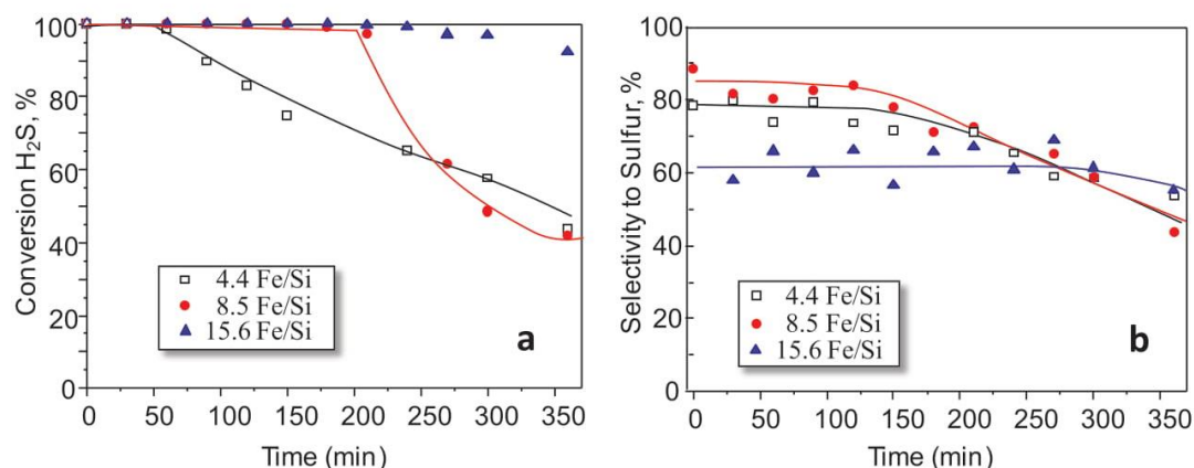
Fig. 8. Variation of \text{H}_2\text{S} conversion (a) and selectivity to sulfur (b) with time on stream achieved during the partial oxidation of \text{H}_2\text{S} over \text{xFe/Si} catalysts. Reaction conditions in text, ( \text{W/F} = 65.2 \text{ g}_{\text{cat}} \text{ h mol}^{-1} ).
