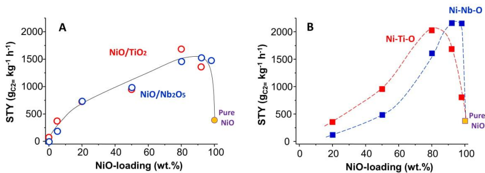
Figure S1. Ethylene Space Time Yield as a function of NiO-loading for diluted (A) or promoted (B) NiO catalysts.
