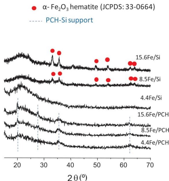
Fig. 1. XRD patterns of xFe/PCH and xFe/Si catalysts.
