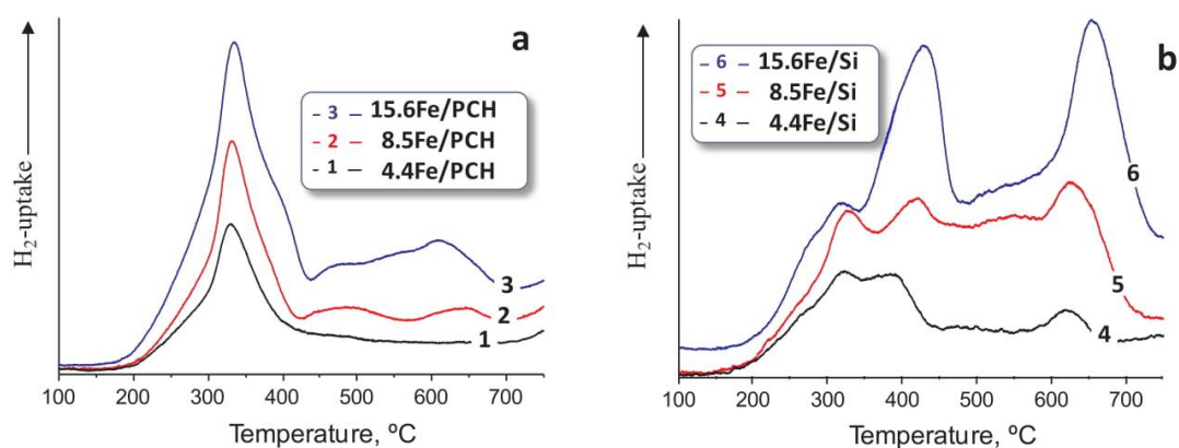
Fig. 3. TPR-H 2 profiles of xFe/PCH (a) and xFe/Si (b) catalysts.
