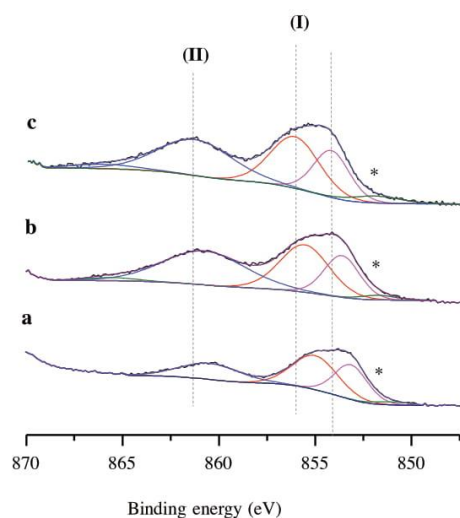
Fig. 5. Ni 2p core level spectra of the 20% wt. NiO-TiO 2 catalysts: a) 20Ni-A, b) 20Ni-B and c) 20Ni-C.
