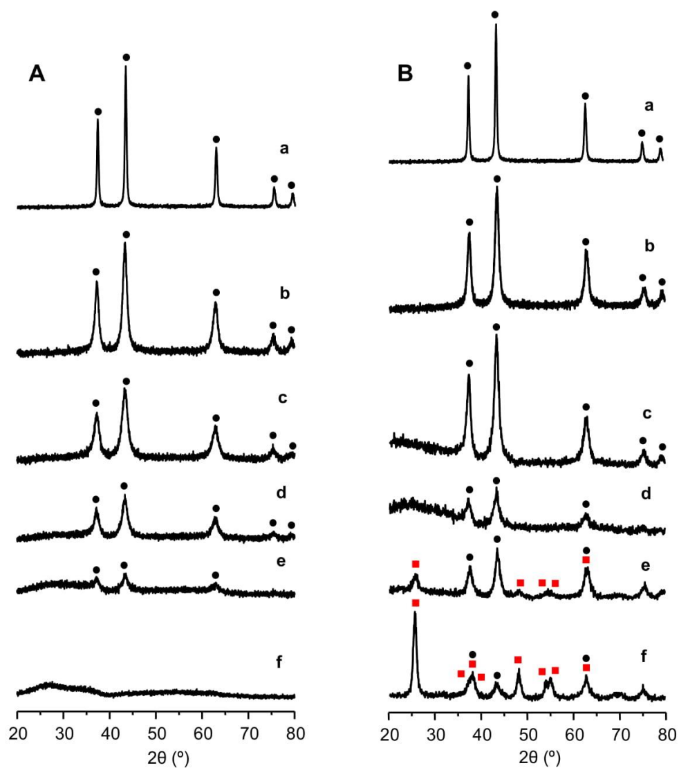
Figure S4. XRD patterns of Nb- (A) and Ti- (B) promoted NiO catalysts. a) NiO; b) 97Ni-Nb-O, 98Ni-Ti-O; c) 92Ni-Nb-O, 92Ni-Ti-O; d) 50Ni-Nb-O, 50Ni-Ti-O; e) 20Ni-Nb-O, 20Ni-Ti-O. Symbols: (●) NiO; (■) TiO 2 -anatase.
