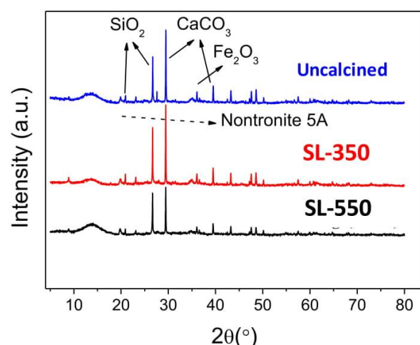
Fig. 1. X-ray diffractograms of the dry sludge (uncalcined) and the two thermally treated materials: sludge ( 350^\circ\text{C} ) and sludge ( 550^\circ\text{C} ).
