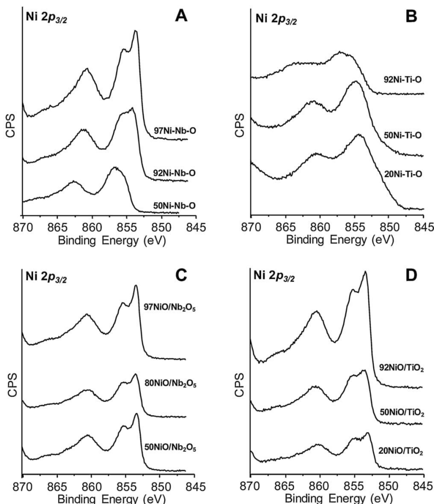
Fig. 4. Ni 2p_{3/2} core level spectra of promoted and diluted NiO catalysts. A) Ni-Nb-O series. B) Ni-Ti-O series. C) \text{NiO}/\text{Nb}_2\text{O}_5 series. D) \text{NiO}/\text{TiO}_2 series.
