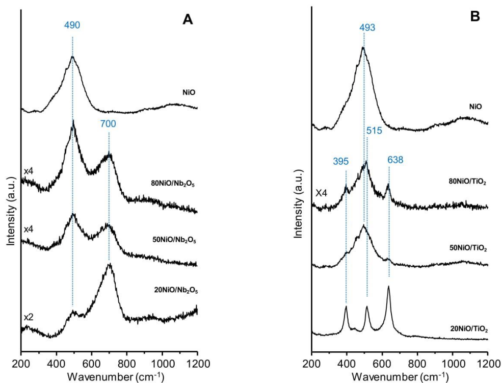
Figure S6. Raman spectra of Nb 2 O 5 - (A) and TiO 2 - (B) diluted NiO catalysts.
