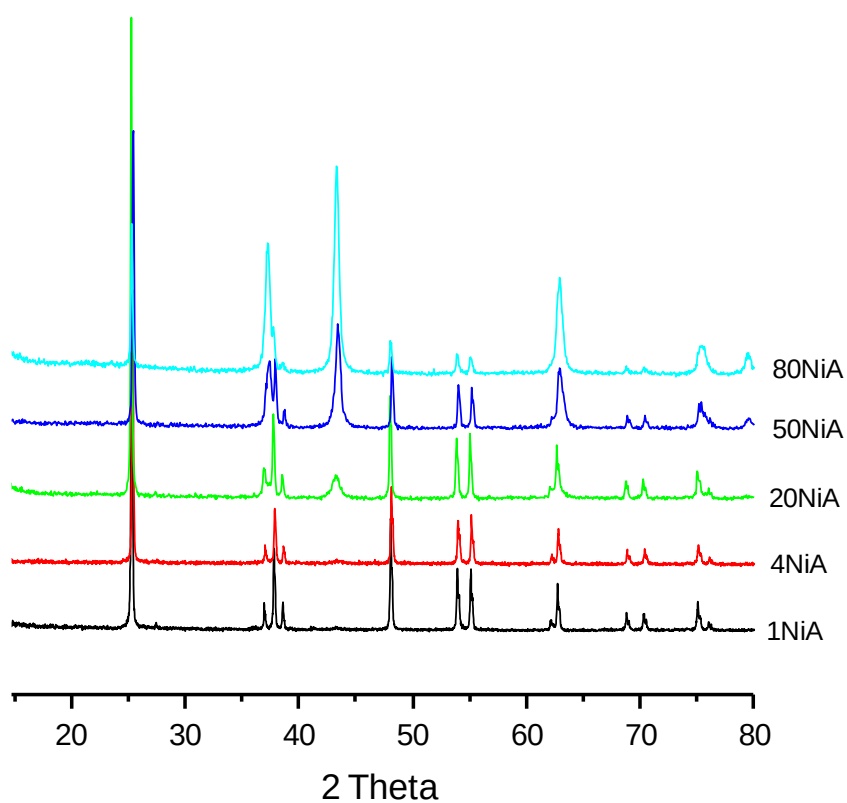
Figure S1. XRD patterns of NiO/TiO 2 catalysts (A-series).
