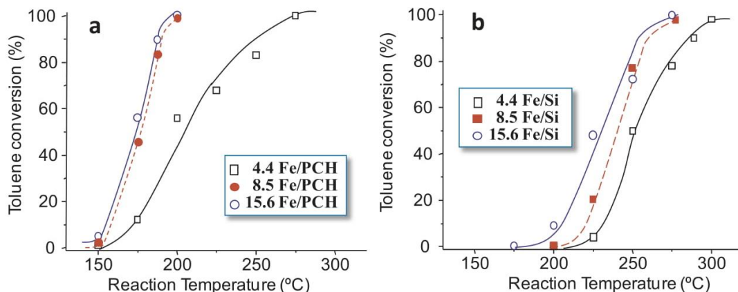
Fig. 6. Variation of toluene conversion with reaction temperature achieved during the combustion of toluene over x\text{Fe}/\text{PCH} (a) or x\text{Fe}/\text{Si} (b) catalysts. Reaction conditions in text.
