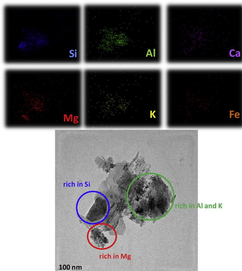
Fig. 3. TEM image with its corresponding XEDS analysis for Si, Al, Ca, Mg, K and Fe of sample SL-550 (ferric sludge calcined at 550 °C).
