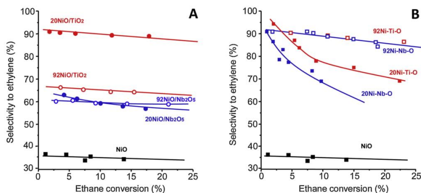
Fig. 2. Variation of the selectivity to ethylene with ethane conversion during the ODH of ethane for selected diluted (A) and promoted (B) NiO catalysts. Reaction conditions in text. Temperature = 450 °C.
