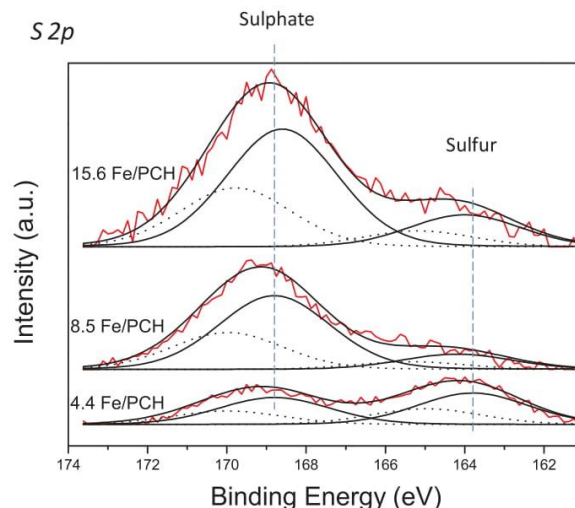
Fig. 9. S 2p core level spectra of iron oxide catalysts supported on PCH.
