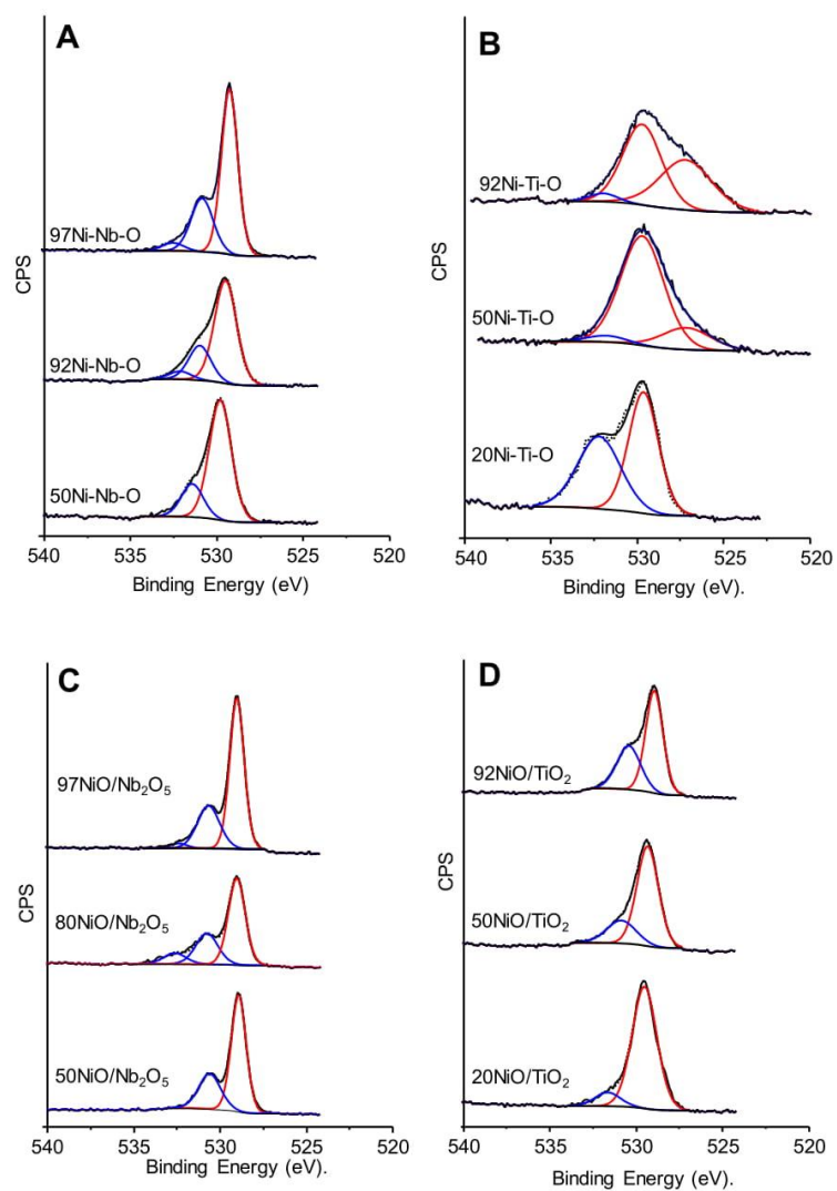
Figure S8. Deconvoluted O 1s core level spectra of promoted and diluted NiO catalysts.
