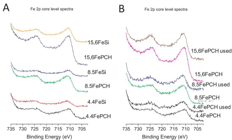
Fig. 4. Fe 2p core level spectra of A) iron oxide supported on a conventional amorphous silica and on the porous clay heterostructure (PCH) and B) iron oxides supported on PCH before and after use in \text{H}_2\text{S} oxidation (reaction conditions in text).
