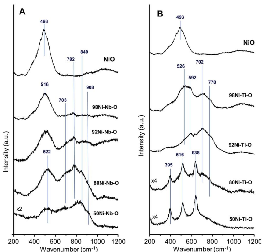
Fig. 3. Raman spectra of Nb- (A) and Ti- (B) promoted NiO catalysts.
